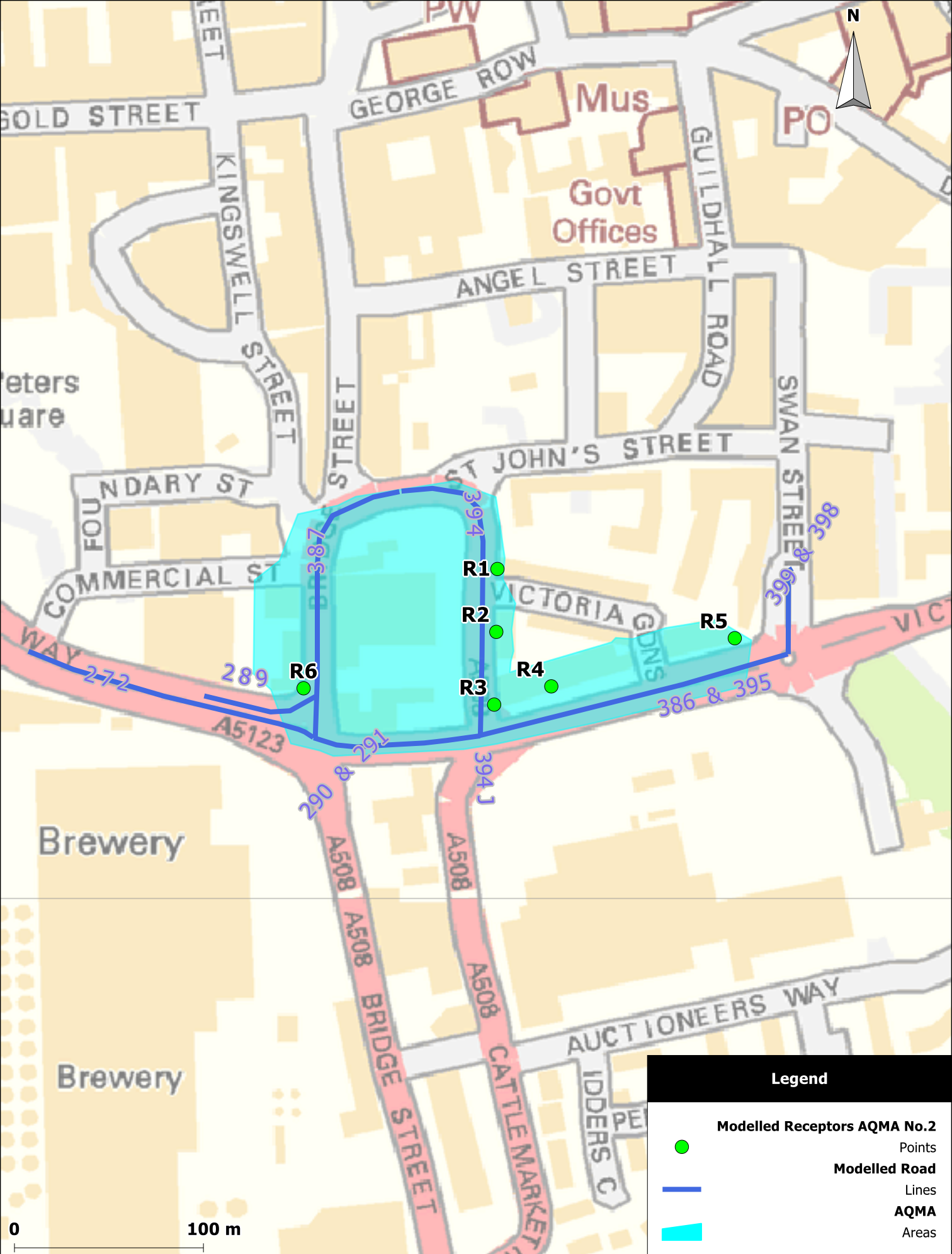
Figure 9.9: Local Operational Impacts - Northampton AQMA No.2, Victoria Promenade
